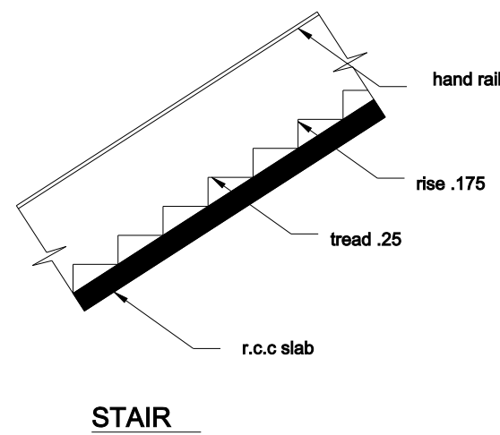
STAIR
