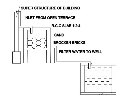
RAINWATER HARVESTING
