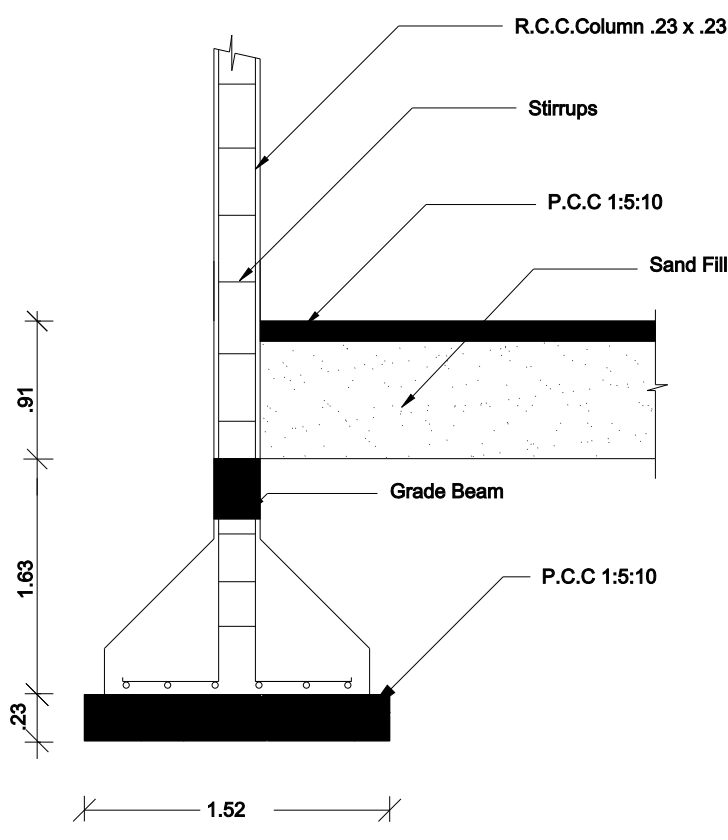
COLUMN DETAIL
