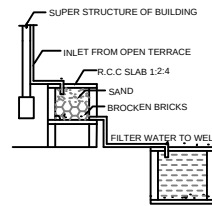
DETAILS OF FILTER BED & WELL NTS
