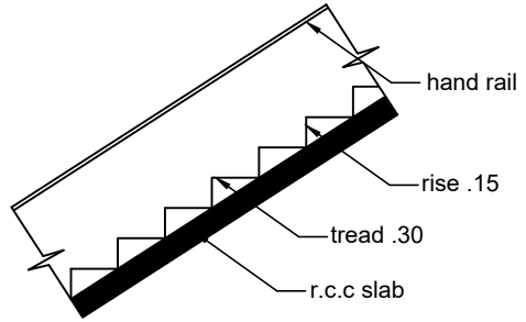
STAIR
