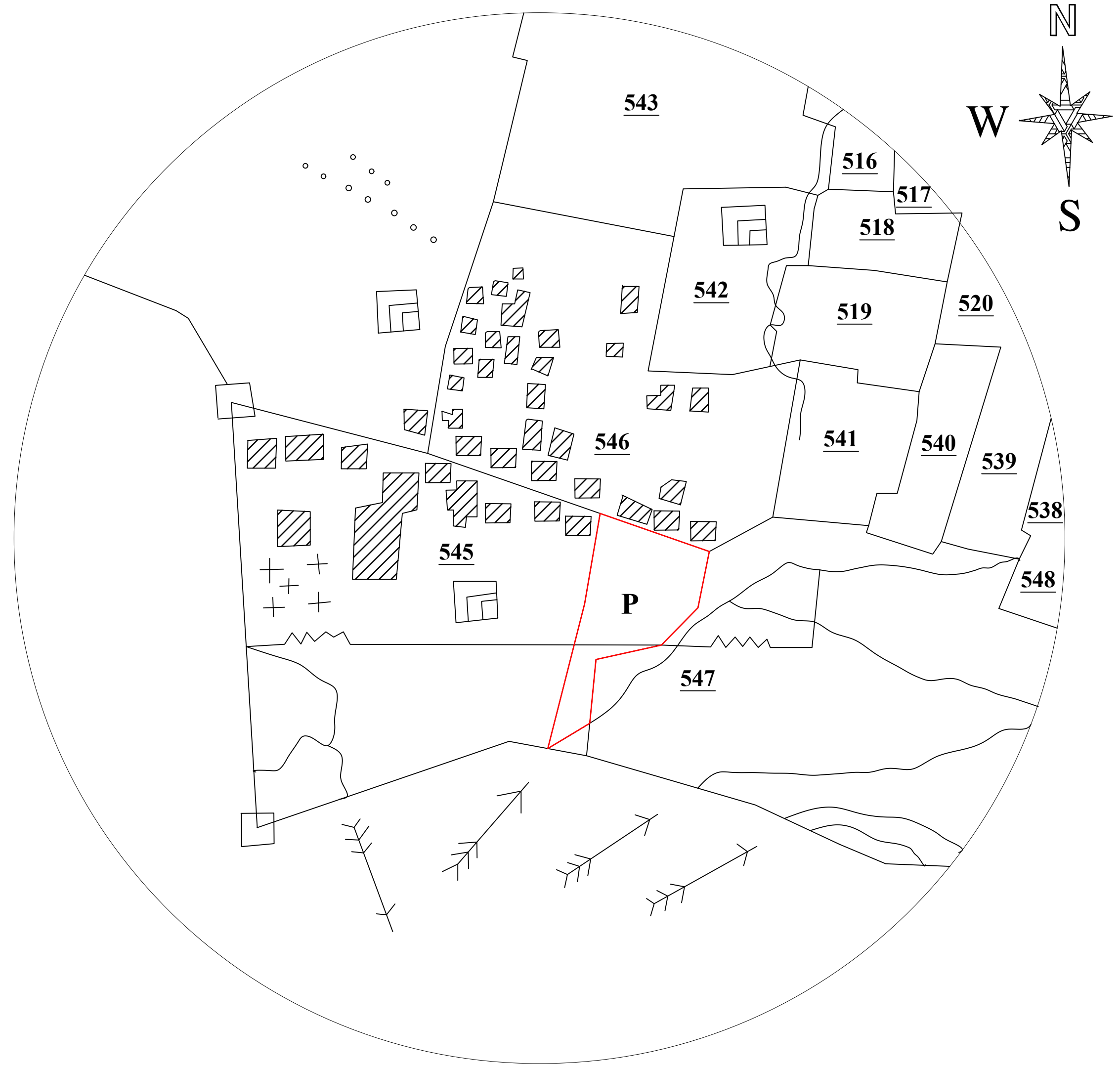
TOPO PLAN
