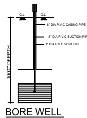
BORE WELL
