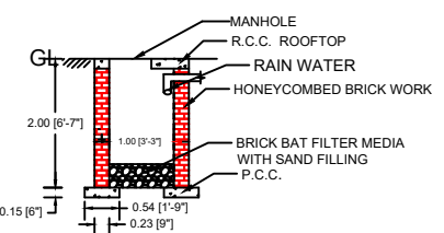
SECTION ON O - P
