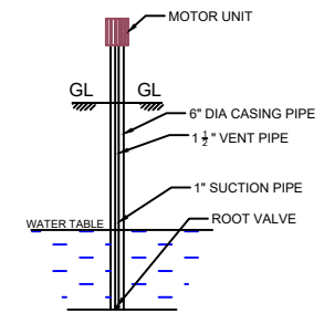
SEC.OF BOREWELL
