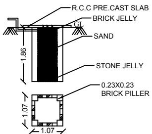
PLAN AND SECTION OF RAINWATER COLLECTION WELL
