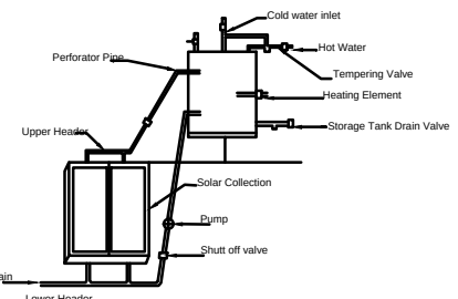
details of solar water Heater (NTS)
