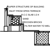
RAINWATER HARVESTING
