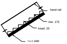
STAIR
