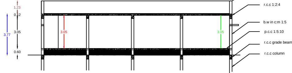
SECTION ON XY
