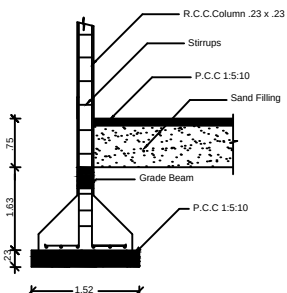
COLUMN DETAIL
