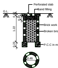
PERCOLATION PIT FOR 30 Sq.m. (Scale:- 1:50)
