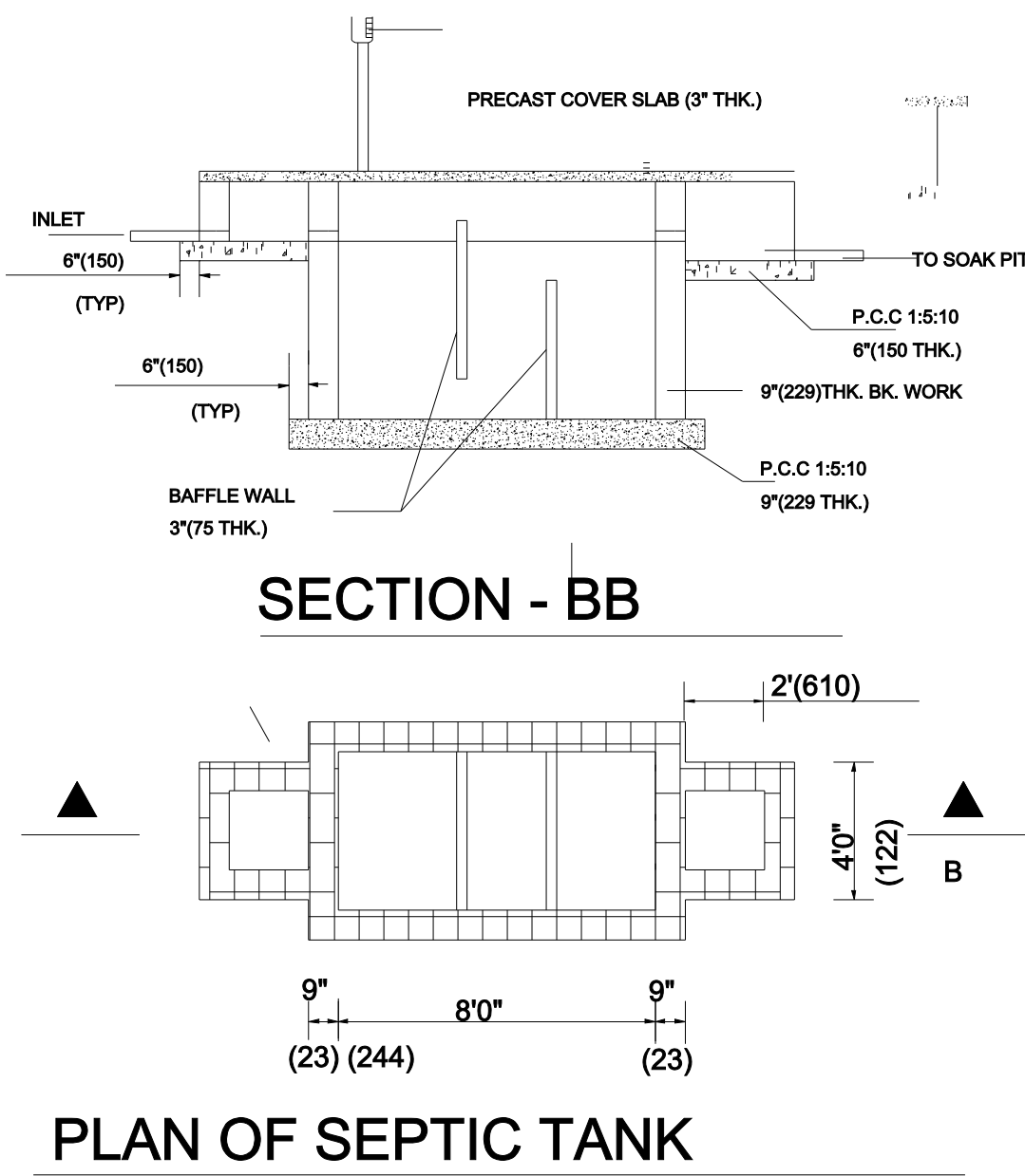
PLAN OF SEPTIC TANK
