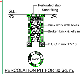
PERCOLATION PIT FOR 30 Sq. m.
