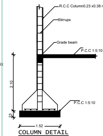
COLUMN DETAIL
