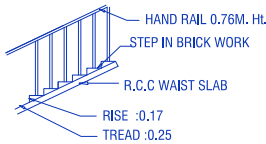
STAIR CASE DETAIL
