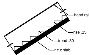
STAIRCASE
