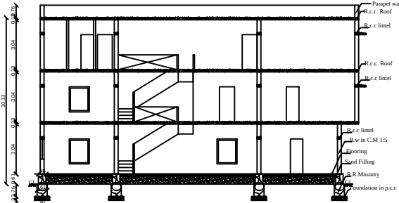
SECTION A&B
