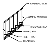
STAIR DETAIL
