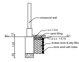
PLINTH BOUNDARY PERCOLATION PIT
