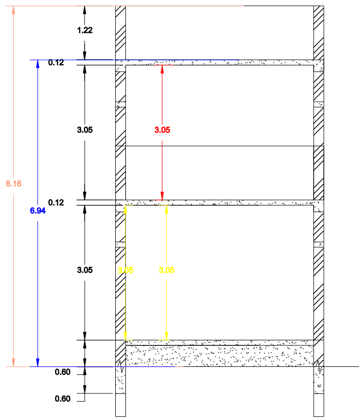
SECTION
