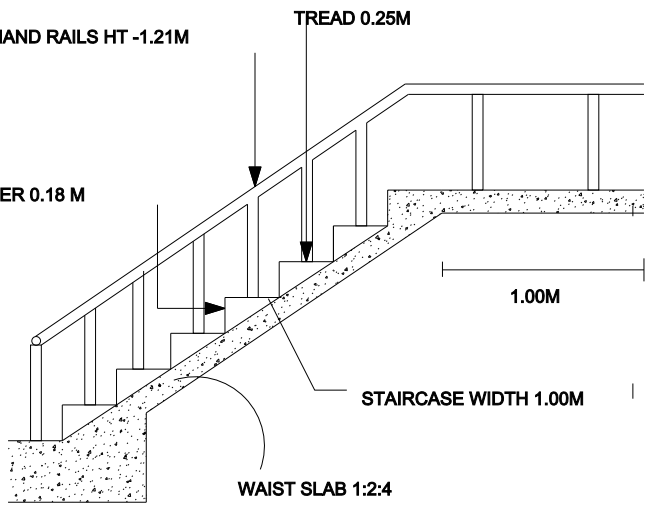
STAIRCASE DETAILS
