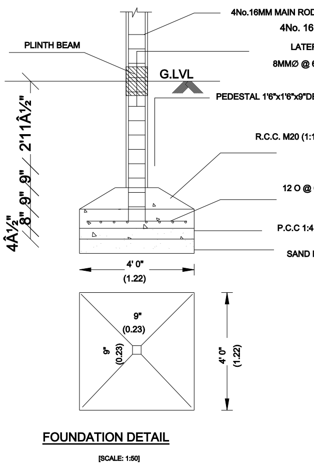
FOUNDATION DETAIL
