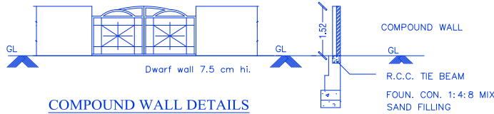
SECTION
