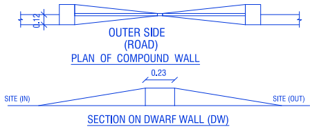
SECTION ON DWARF WALL (DW)
