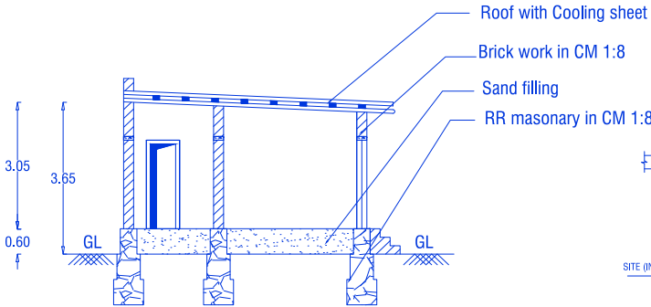
CROSS SECTION ON 'AB'
