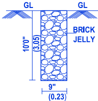
PERCUSSION PIT
