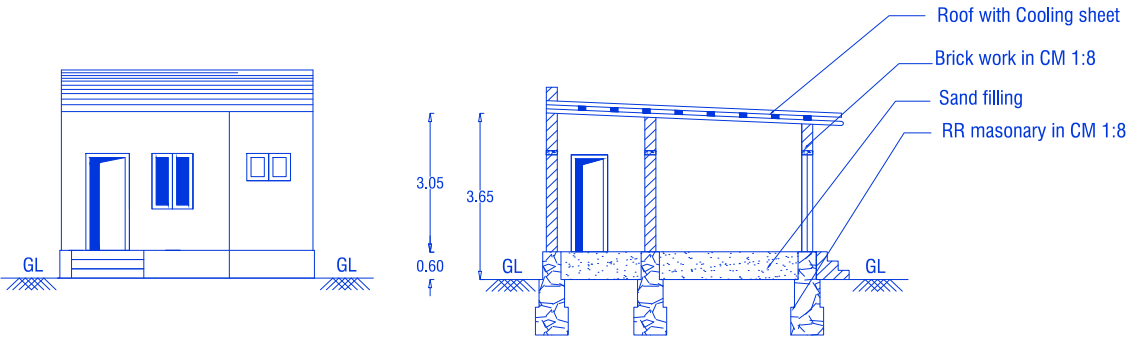
FRONT ELEVATION
