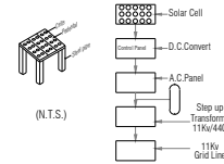
SOLAR SYSTEM FLOW DIAGRAM (7 - NOS PROVIDED)
