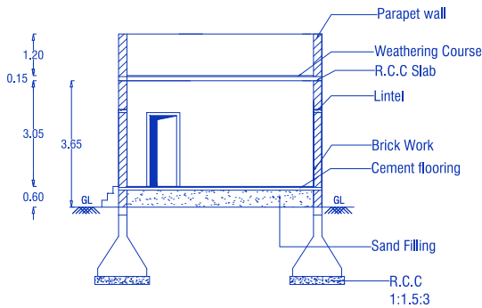
CROSS SECTION ON 'AB'
