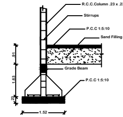
COLUMN DETAIL
