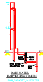
RWH_CAPACITY: L=1000LTRS
