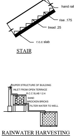
RAINWATER HARVESTING
