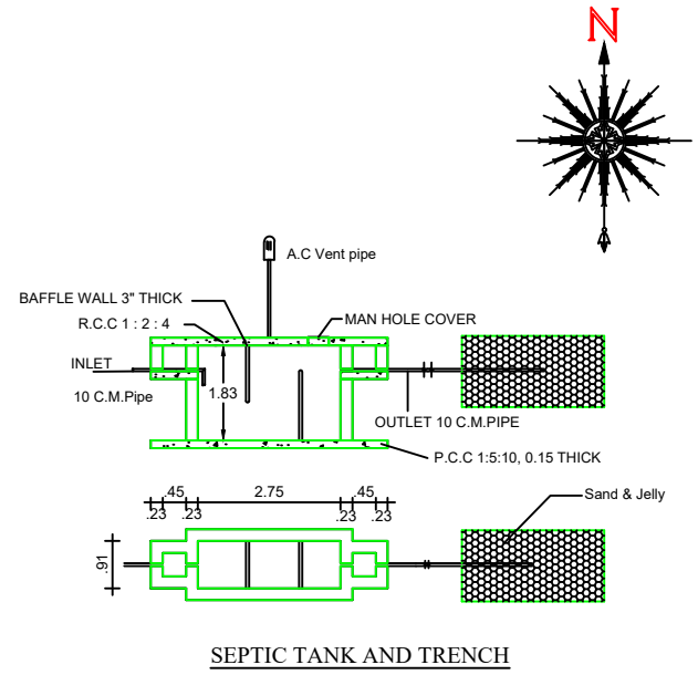
SEPTIC TANK AND TRENCH
