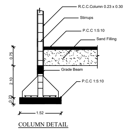
COLUMN DETAIL
