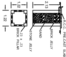
PLAN & SECTION OF RAIN WATER COLLECTION WELL
