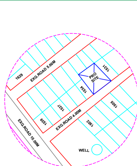
TOPO PLAN NOT TO SCALE
