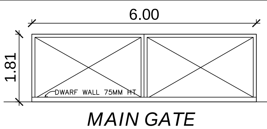
MAIN GATE
