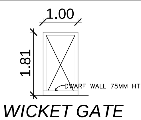
WICKET GATE
