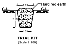
TRIAL PIT (Scale 1:100)
