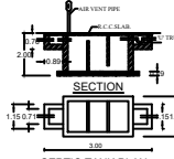
SEPTIC TANK PLAN
