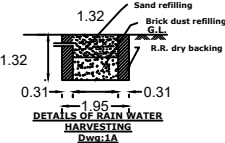
DETAILS OF RAIN WATER HARVESTING Downspout
