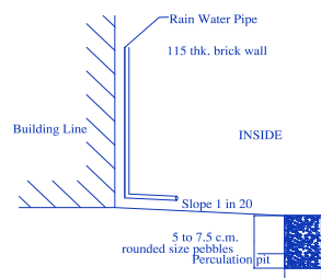
PERCOLATION PIT
