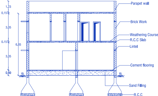
CROSS SECTION ON 'AB'
