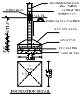
FOUNDATION DETAILS
