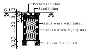
PERCOLATION PIT FOR 30 Sq. m. (Scale:- 1:50)
