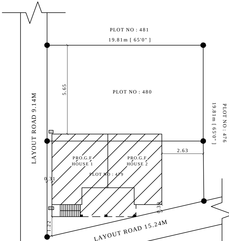
SITE PLAN
