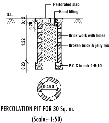
PERCOLATION PIT FOR 30 Sq. m.
