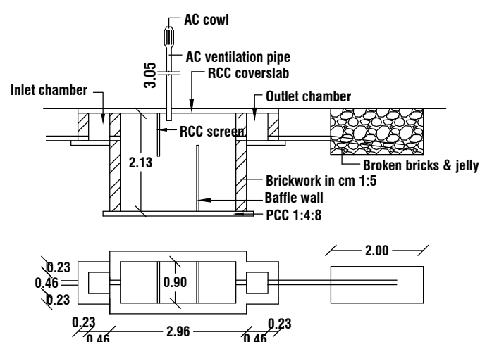
TOPO PLAN
