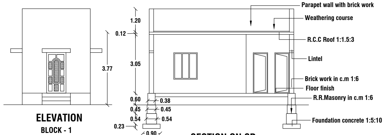
SECTION ON CD BLOCK - 1
