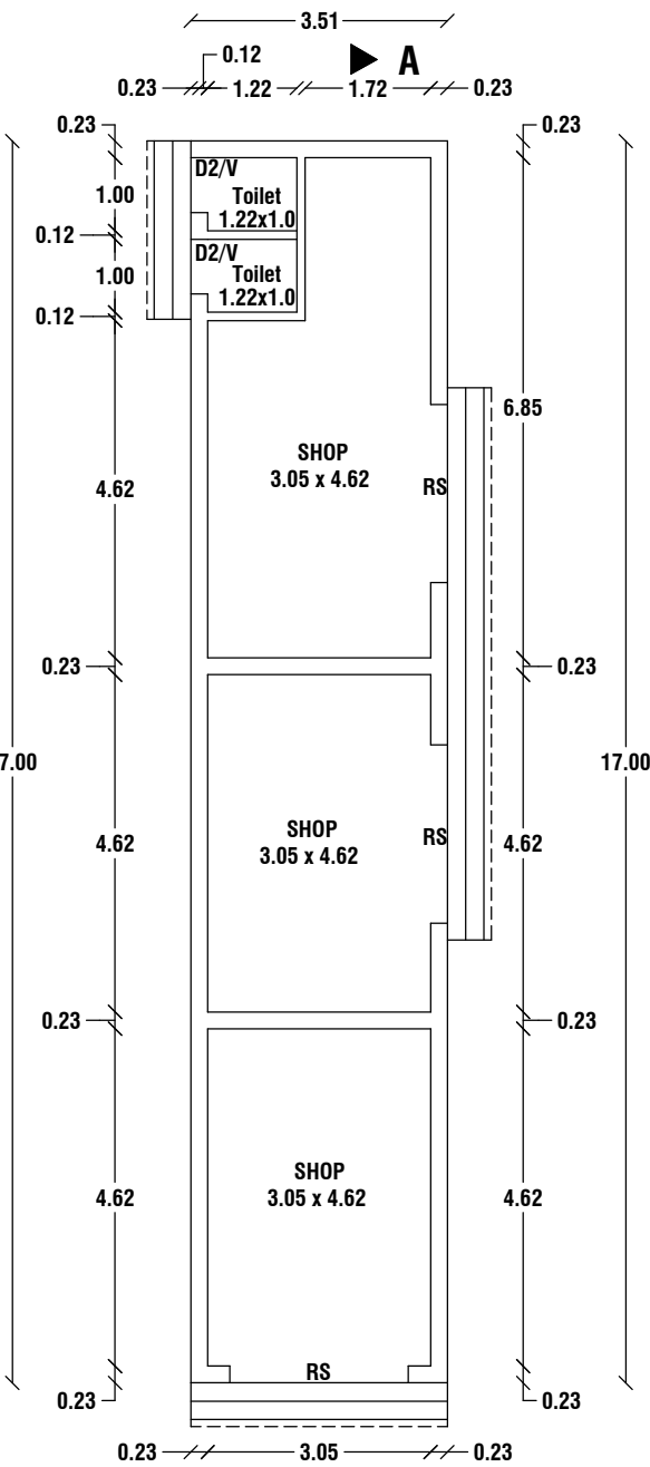
PLAN BLOCK - 2
