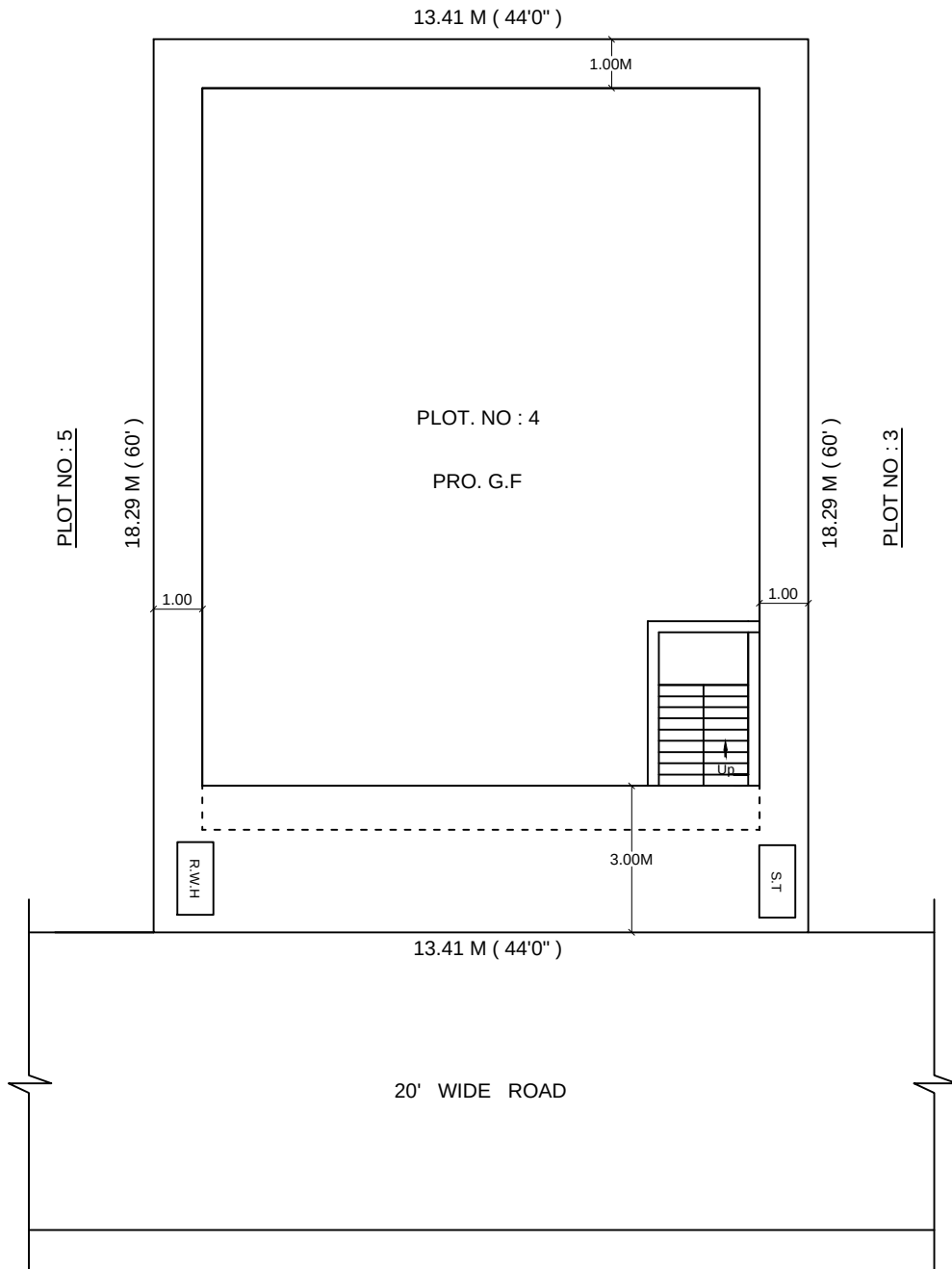
SITE PLAN
