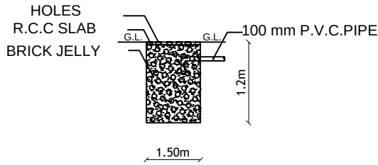
SECTION OF RAIN WATER PIT
