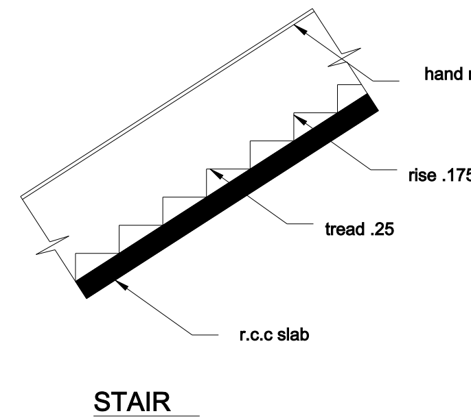
STAIR
