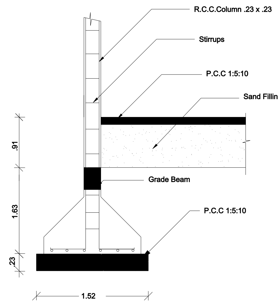
COLUMN DETAIL
