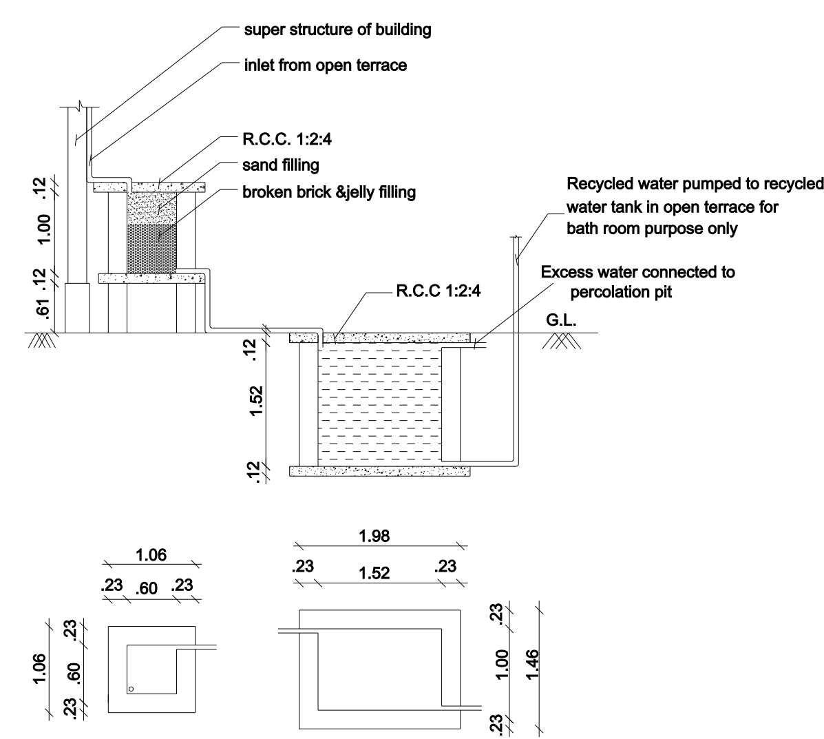
Sump and Filter Bed
