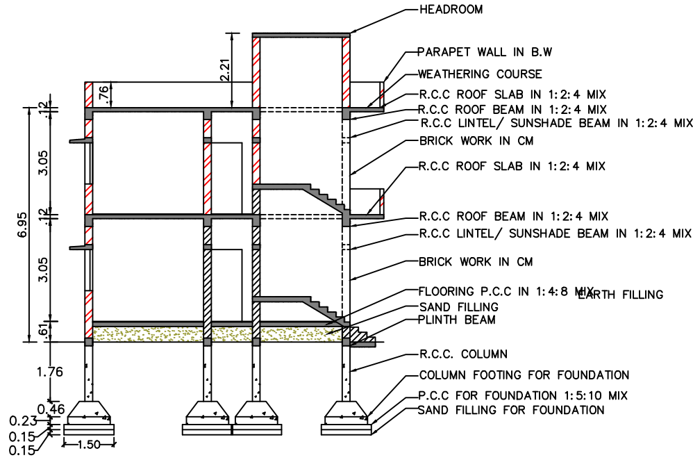
SECTION ON-AA
