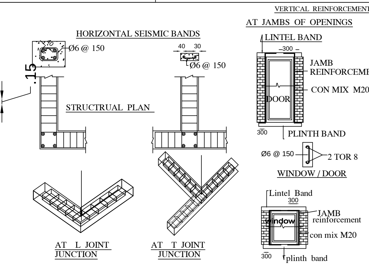
STRUCTURAL PLAN
