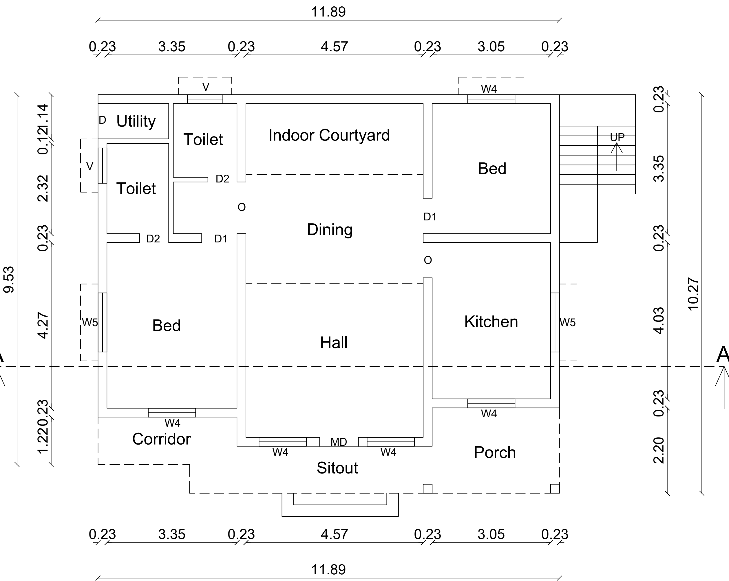
PLAN
