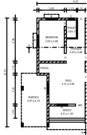
EXG. GROUND FLOOR
