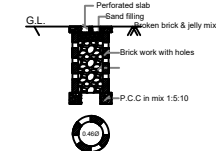
PERCOLATION PIT FOR 30 Sq. m.
