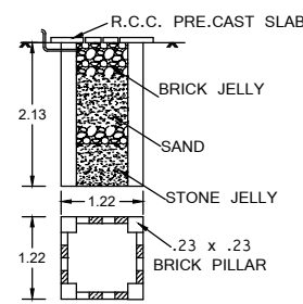
PLAN & SECTION OF RAIN WATER COLLECTION WELL
