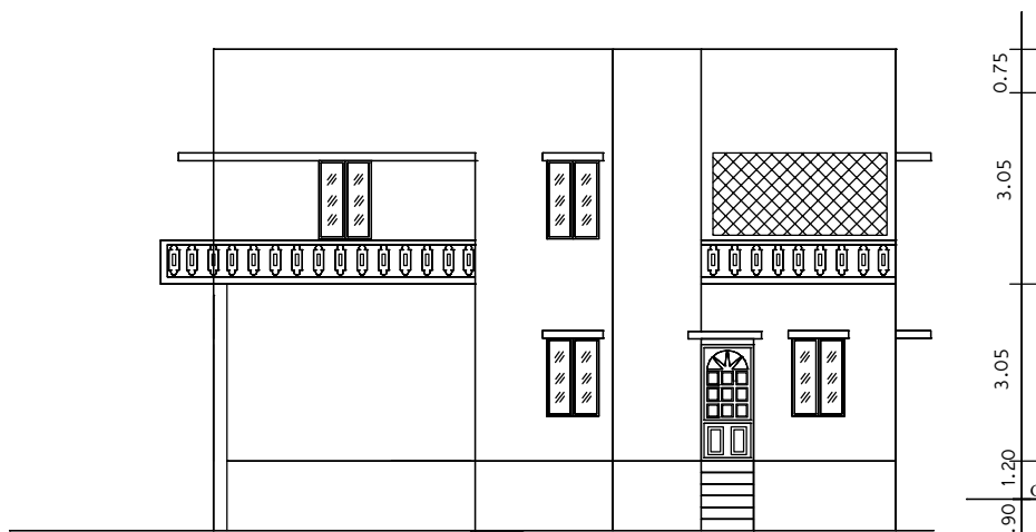
FRONT ELEVATION
