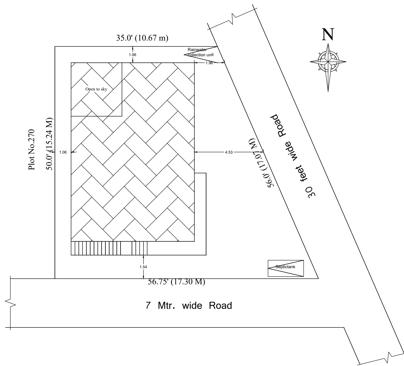
SITE PLAN
