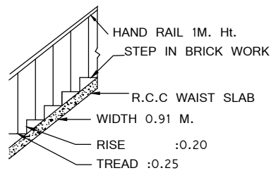
STAIR DETAIL
