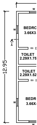
PROPOSED GROUND FLOOR PLAN
