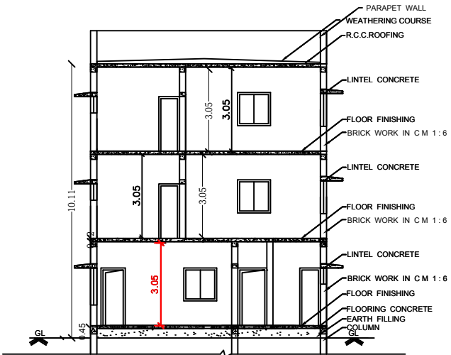
SECTION VIEW
