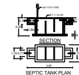
SEPTIC TANK PLAN
