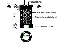
PERCOLATION PIT FOR 30 Sq. m. (Scale:- 1:50)
