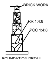
FOUNDATION DETAIL NOT TO SCALE
