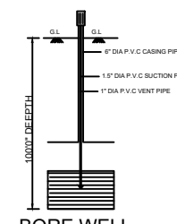
BORE WELL
