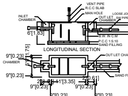
SEPTIC TANK:
