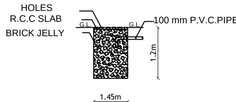
SECTION OF RAIN WATER PIT
