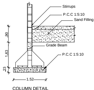
COLUMN DETAIL
