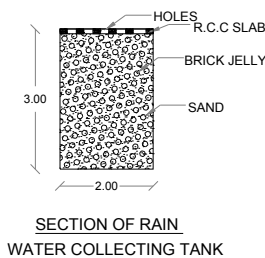
SECTION OF RAIN WATER COLLECTING TANK
