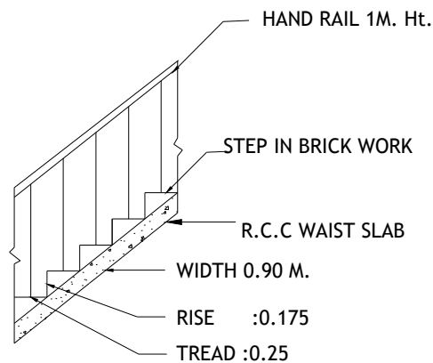
STAIR DETAIL
