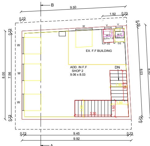
PRO.ADDITIONAL FIRST FLOOR PLAN
