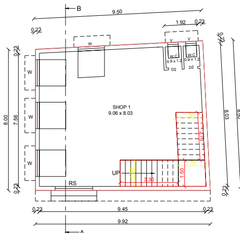
EX. GROUND FLOOR PLAN
