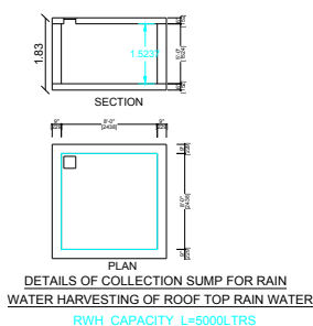
PLAN DETAILS OF COLLECTION SUMP FOR RAIN WATER HARVESTING OF ROOF TOP RAIN WATER RWHP_CAPACITY_1X500X.TRS
