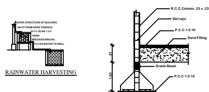
COLUMN DETAIL
