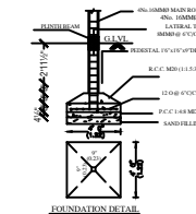
FOUNDATION DETAIL
