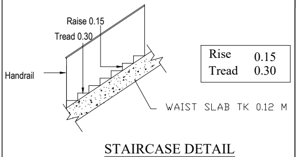
STAIRCASE DETAIL
