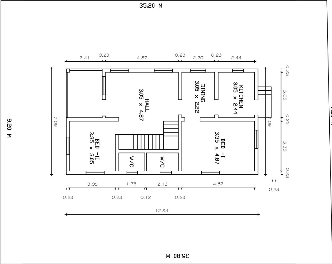
SITE CUM GROUND FLOOR PLAN
